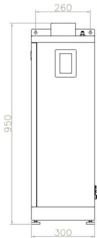
FRONT VIEW
